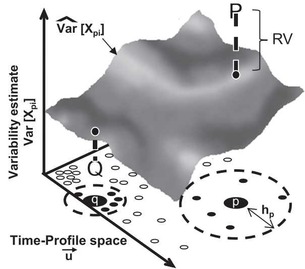
Fig. 1. RV. A conditional variance estimate ( \widehat{\text{Var}}[X_{pi}] ) is computed for a feature, X , at every point in the feature space based on the nearby data points. For points of interest (corresponding to proteins, indicated by p and q ), a bandwidth parameter h_p is computed based on the density of points (proteins with similar localization patterns) in that region of the space. The RV compares the conditional variance estimate (surface) to the observed variability (bold P and Q). In this example, the observed variability is high for protein p (P is above the surface) and is low for q (Q is below the surface)
